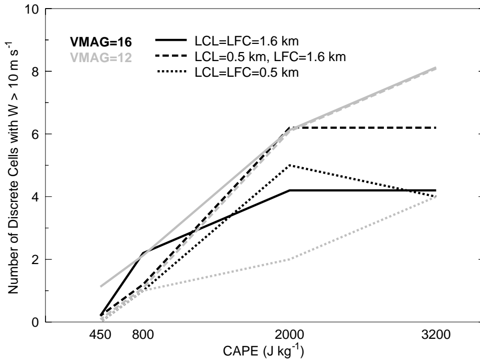
Figure 12. Number of discrete updrafts of at least 10 \text{ m s}^{-1} in a subset of the COMPASS simulations, counted at the last model timestep (120 min) and at 2 km AGL. Gray lines denote VMAG = 12, and the black lines VMAG = 16. Line styles denote the three possible combinations of LCL and LFC, and each line connects simulations with every other environmental parameter held constant except for CAPE. Traces are slightly offset from their integer values for readability.
