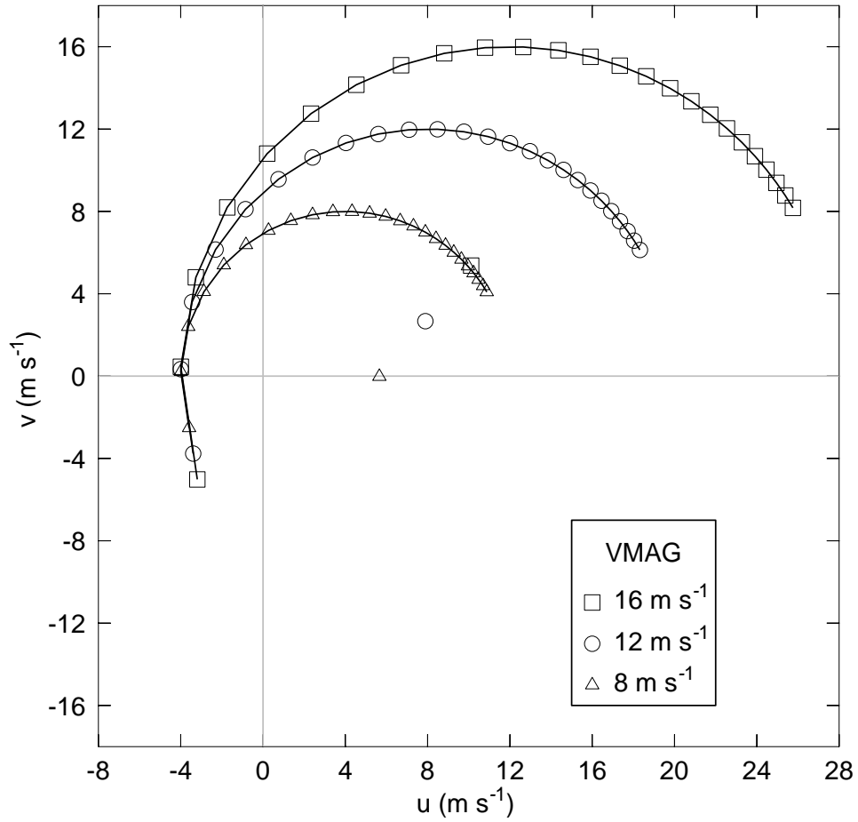
Figure 2. Sample hodographs (translated) for use in the COMPASS simulations. The hodograph radius (VMAG) is either 8, 12, or 16 m s -1 . Each hodograph is translated so that the u wind at 0.5 km is -4 m s -1 . Symbols are given every 500 m, from the surface to 12 km AGL. A storm-motion estimate using the method of Bunkers et al. (2000) is also shown for each hodograph.
