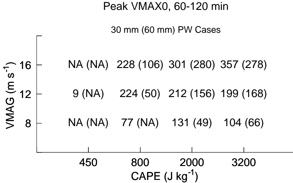
Figure 10. As in Fig. 5, but for peak second-hour VMAX0 ( 10^4 \text{ s}^{-1} ).
