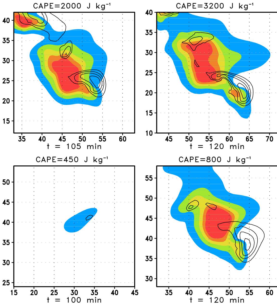
Figure 7. As in Fig. 6, but for VMAG = 16 m s -1 .
