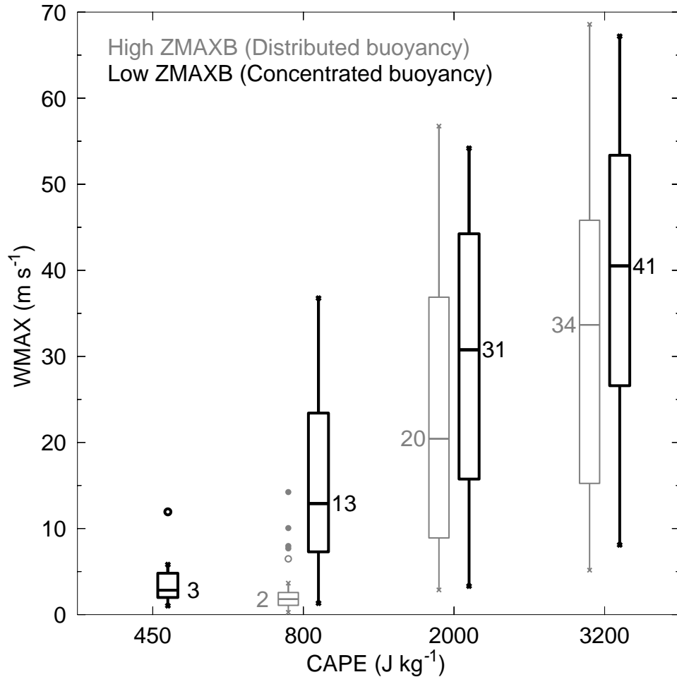
Figure 8. Boxplots illustrating the influence of changing the vertical distribution of buoyancy on second-hour WMAX. Simulations with low ZMAXB are shown in black, high ZMAXB in light gray. All 225 experiments are shown. Each box plot shown consists of 36 unique experiments for CAPE \geq 800 , and 9 experiments for CAPE = 450. No simulations were conducted at CAPE = 450 and “high” ZMAXB. The box edges show the first (q1) and third (q3) quartiles, and the whiskers extend to the farthest data points that are still within a distance of 1.5 interquartile ranges from q1 and q3. Outliers beyond the whiskers are shown, in open circles up to a distance of three interquartile ranges beyond q1 or q3, and in closed circles beyond that. The median WMAX for each distribution is also shown.
