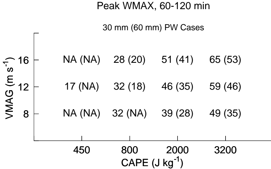
Figure 5. The peak second-hour WMAX ( \text{m s}^{-1} ) for persistent right-moving storms. Binned by CAPE and VMAG as in Fig. 4, with further stratification also given by environmental PW. Each table entry is the average of all experiments that produce persistent storms with those CAPE, VMAG, and PW values. The average value for all storms with “low” PW (30 mm) is given at left, and for “high” PW (60 mm) in parentheses. Only the 140 persistent storms (whose distribution is shown in Fig. 4) are included. “NA” means no persistent storms occurred in any of the simulations with those values of CAPE, VMAG, and PW. No simulations were conducted at CAPE = 450 and PW = 60.
