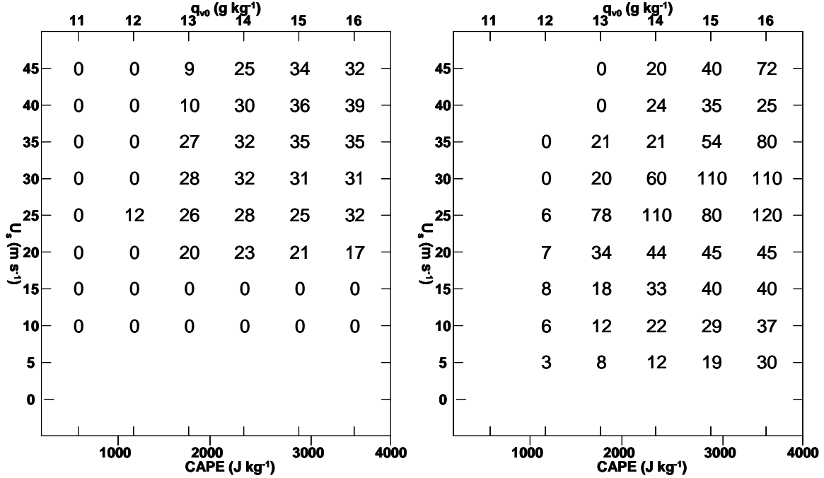
Figure 1. Adaptations of Figs. 10c and 11 of Weisman and Klemp (1982). Maximum vertical velocity at any model level ( \text{m s}^{-1} ; left) and vorticity at 178 m ( 10^{-4} \text{ s}^{-1} ; right) of simulated storms in the WK parameter space study. CAPE is given in units of \text{J kg}^{-1} and in terms of boundary layer mixing ratio, q_{v0} . Wind shear is given as U_s .
