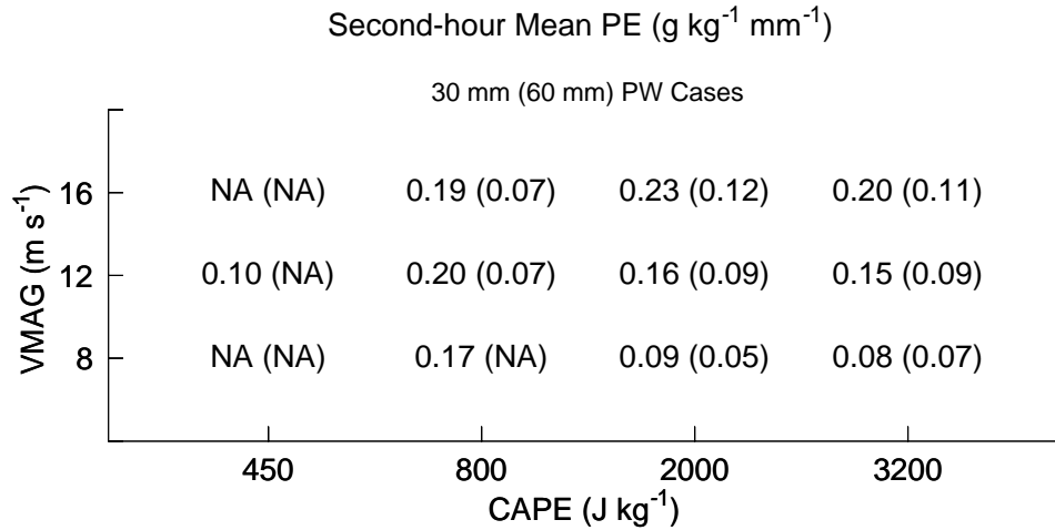
Figure 14. As in Fig. 5, but for mean second-hour precipitation efficiency (PE), defined in the text as RMAX0 divided by PW. For reference, the highest value of PE (in the given units) at any 5-min output time in any of the 225 simulations is 0.33.
