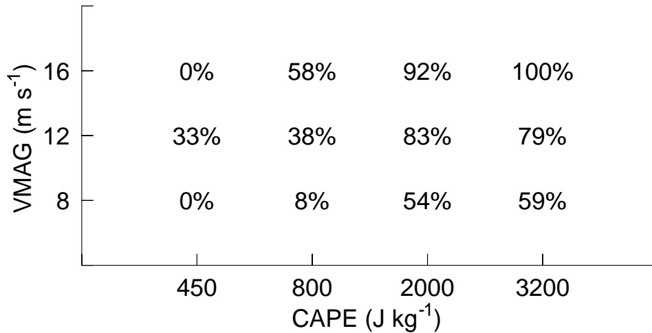
Figure 4. The percentage of experiments with strong, “persistent” storms (as defined in the text) in the COMPASS simulation set, grouped by VMAG (hodograph radius) and CAPE. For CAPE = 450, each entry is comprised of 3 possible experiments; for CAPE \geq 800, 24 experiments are conducted at each combination of CAPE and VMAG. For example, only 2 of 24 simulations (8%) with VMAG = 8 and CAPE = 800 feature a persistent storm.
