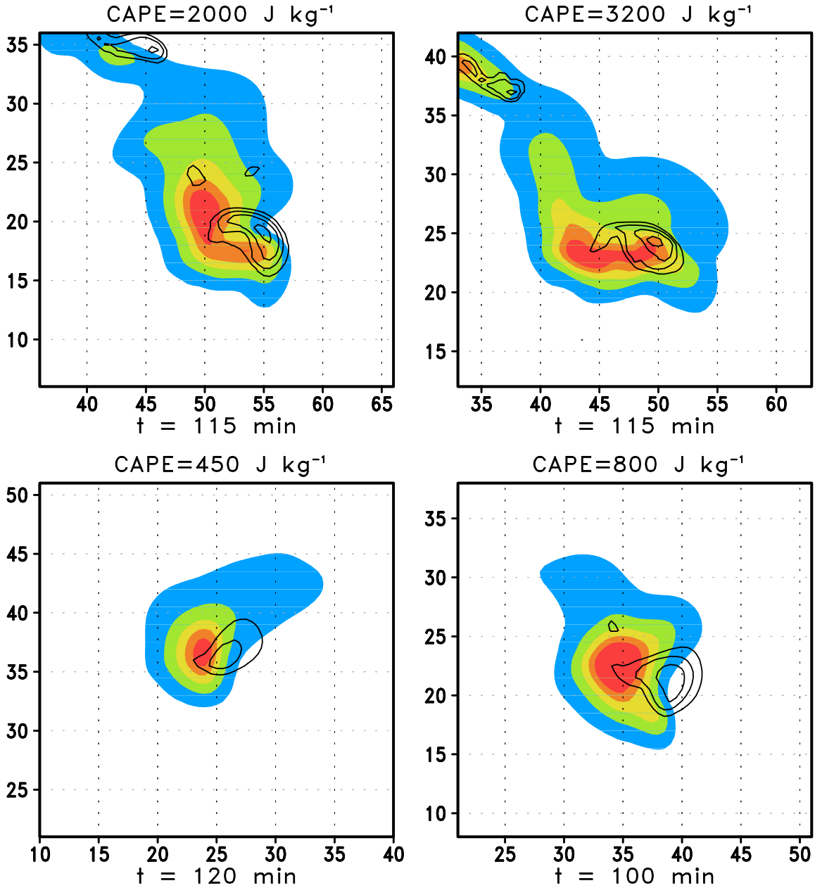
Figure 6. Maps of simulated updraft velocity at 3.5 km (contoured at 5, 10, 15, 20, 25, and 30 m s -1 ) and rainwater mixing ratio at 126 m (shaded at 0.25, 1, 2, 3, and 4 g kg -1 ) for simulations with constant VMAG (12 m s -1 ), low ZMAXB and ZMAXV, LCL = LFC = 1.6 km, and PW = 30 mm. Axes are in km. Each plot is taken from the last 20 min of its simulation, at a time deemed representative of mature storm structure.
