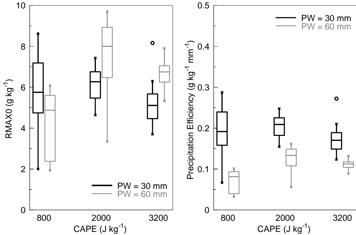
Figure 11. Boxplots (as in Fig. 8) of persistent storm RMAX0, averaged over each experiment's second hour, for 25 sets of three experiments with only CAPE varied from 800 to 3200 J kg -1 . Experiments are further binned by PW. Only one persistent storm occurred in nine simulations produced at CAPE = 450, and it is excluded from the figure.
