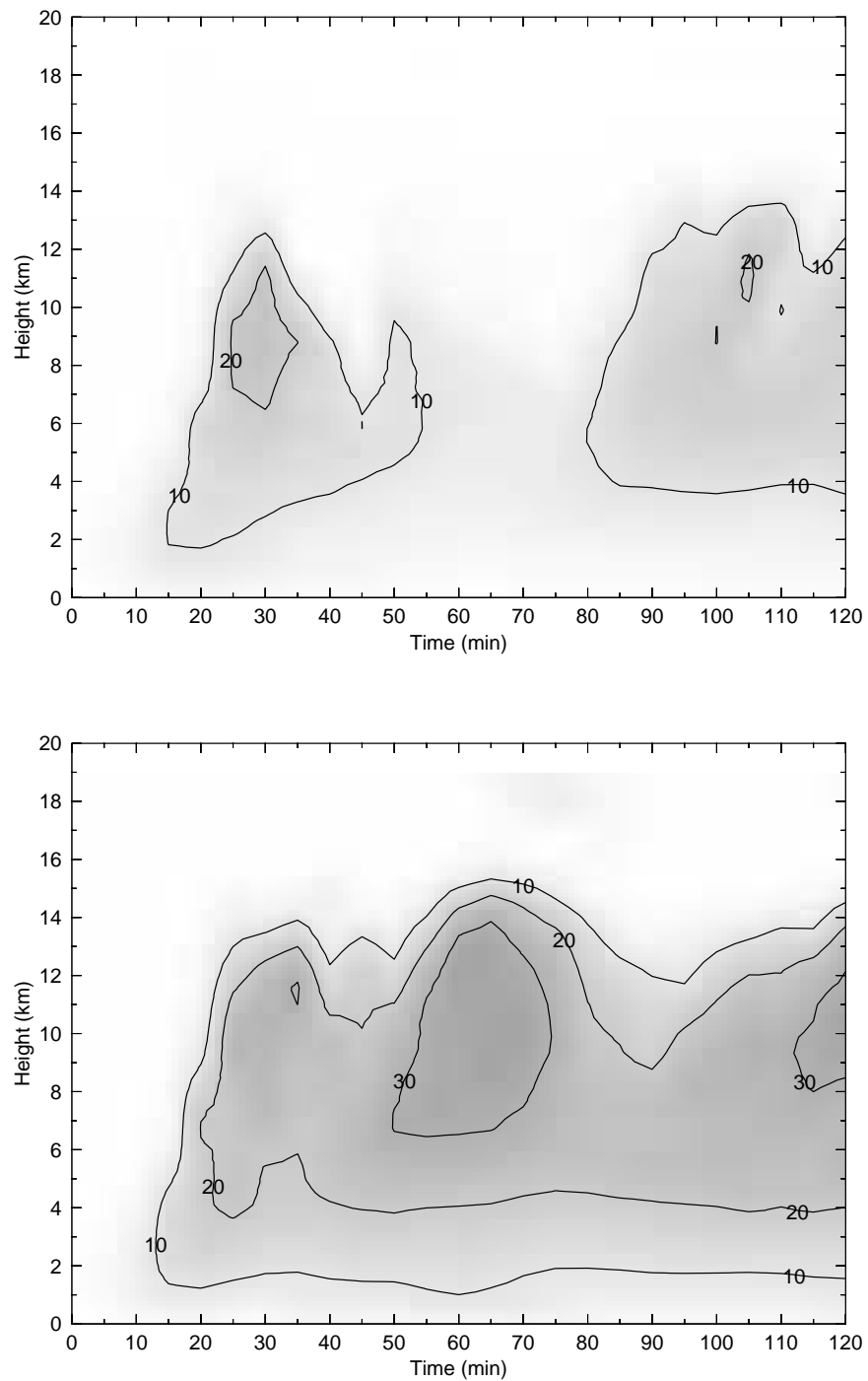
Figure 9. Time-height series of updraft velocity ( W_{MAX} ; m s^{-1} ) for the dominant right-moving storm in the domain of two simulations with only Z_{MAXB} varied. The top panel shows the high- Z_{MAXB} case, and the bottom panel shows the low Z_{MAXB} case. Both simulations have CAPE = 800 J kg^{-1} , VMAG = 16 m s^{-1} , the high value of Z_{MAXV} , LCL = 0.5 km , LFC = 1.6 km , and PW = 30 mm .
