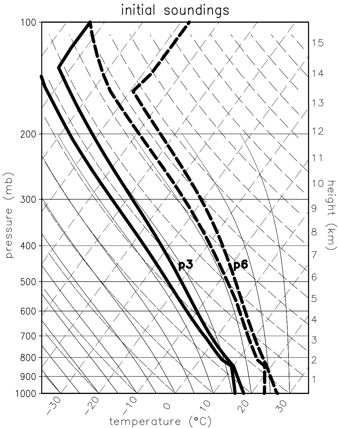
Figure 3. Example initial thermodynamic profiles for two COMPASS simulations. These two sample profiles have \text{CAPE} = 2000 \text{ J kg}^{-1} , \text{LCL} = 1.6 \text{ km} , and \text{LFC} = 1.6 \text{ km} . The solid lines labeled “p3” represent the \text{PW} = 30 \text{ mm} environment, and the dashed lines labeled “p6” represent the \text{PW} = 60 \text{ mm} environment.
