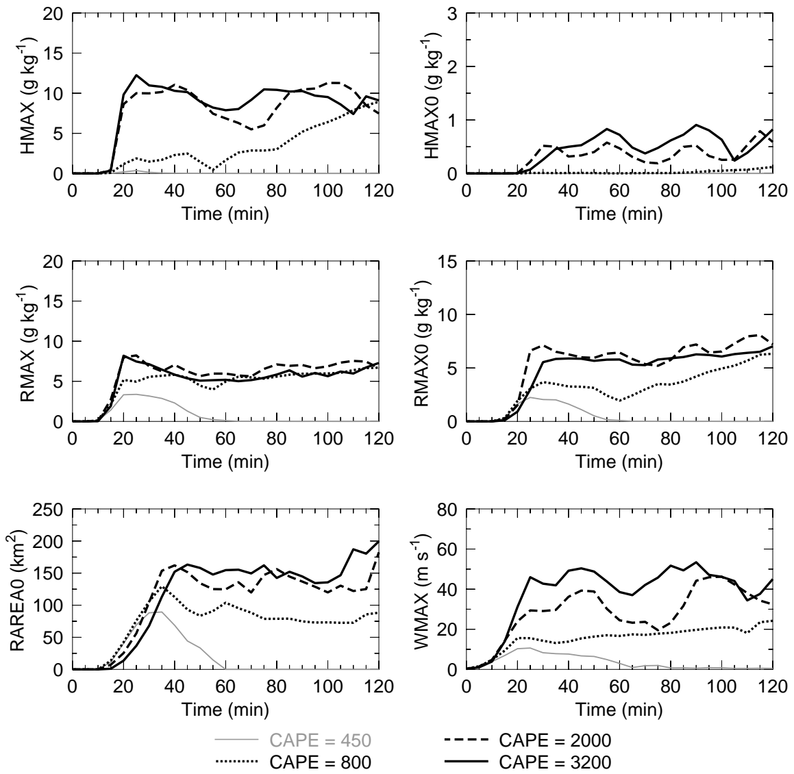
Figure 13. Time series plots of storm properties from four simulations with only CAPE changed. All simulations shown have VMAG = 16 m s -1 , the low value of ZMAXB and ZMAXV, LCL = LFC = 0.5 km, and PW = 30 mm. Acronyms are defined in the text.
